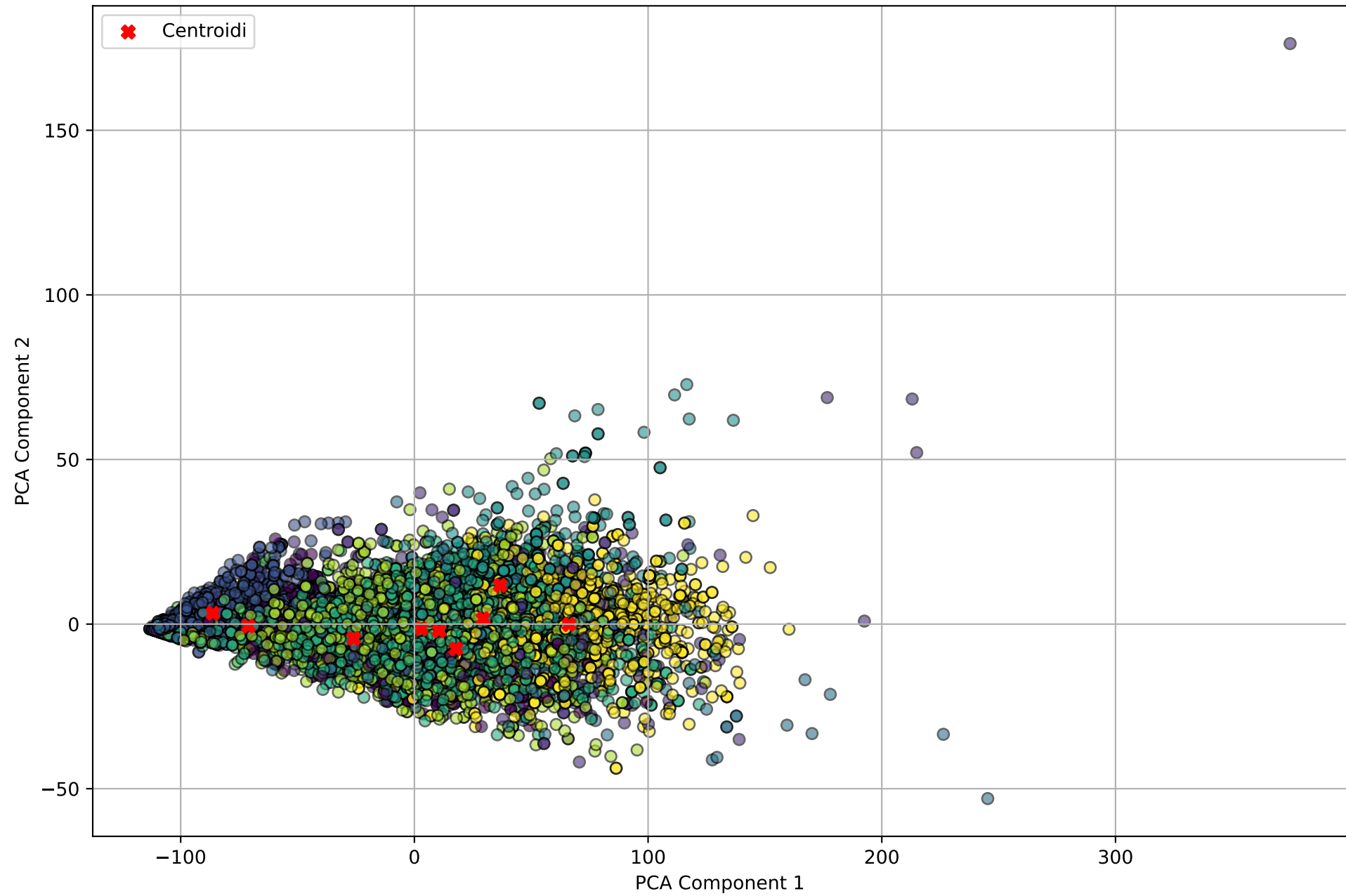
Gaussian_mixtures Clusters in PCA Projection (all wines)
